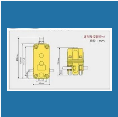
Tower Crane Limit Switch
